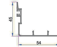
Alm. Kanat Arka Kapama 16051.601.5.1.1.9016
