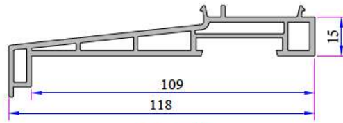
Sill Profile 058.5504
