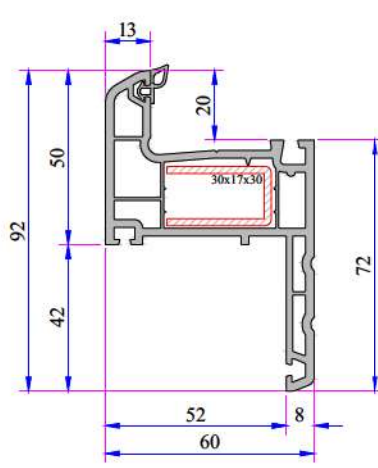
Dekoratif Pervazlı Kasa 42 mm 632.1200 632.1200.PC (with Double Seal)
