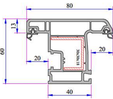
Dekoratif Pervazlı Kasa 42 mm 632.1200 632.1200.PC (with Double Seal)
