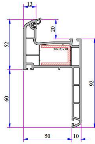
Düz Pervazlı Kasa 60 mm 632.1207 632.1207.PC (with Double Seal)
