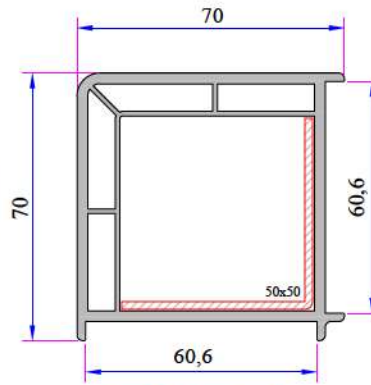
90° Corner Profile 060.5100
