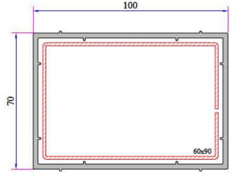
Kutu Profili 70x100mm P.A.070.5202.600.0.00.19
